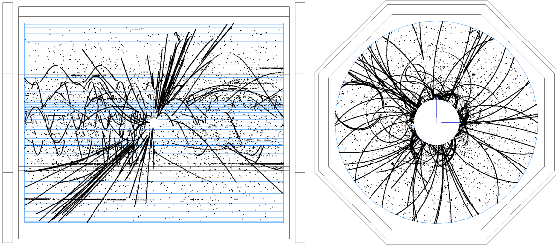
FIGURE 3.2-6. The same event as the previous figure, with the micro-curlier removal algorithm applied. This is the input to the TPC track finding algorithm.
