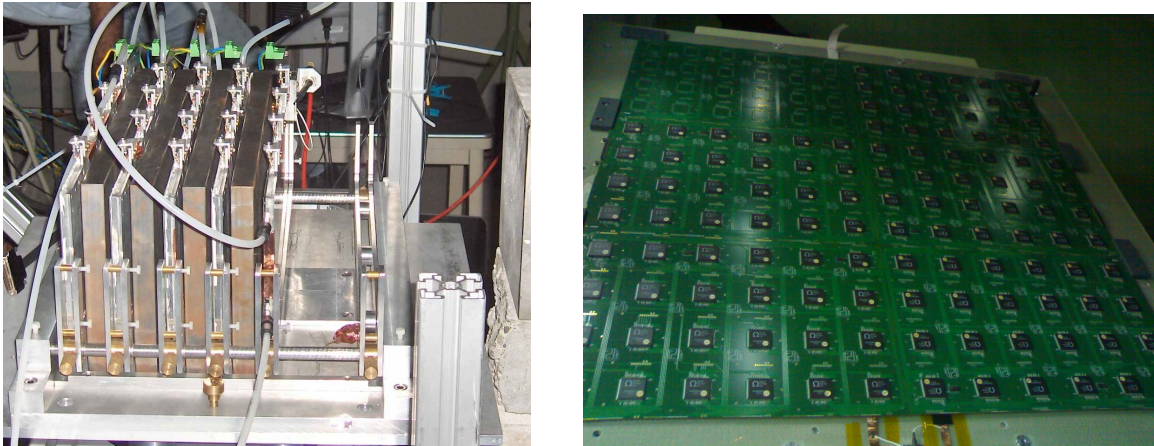
FIGURE 4.4-22. Mini-DHCAL prototype (left); Prototype of a large instrumented GRPC (right).
